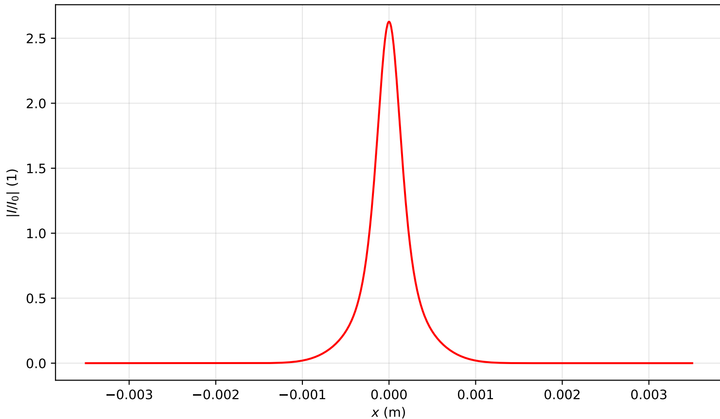
Intensity profile I(x, y = 0, z = 0.716)/I_0 , P_{in}=2.0P_{cr} , artificial time
